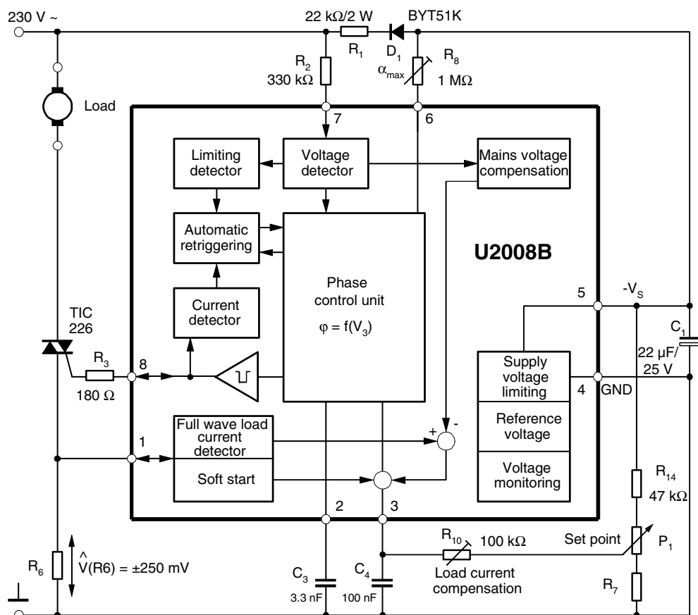
Figure 1-1. Block Diagram with Typical Circuit: Load Current Sensing
